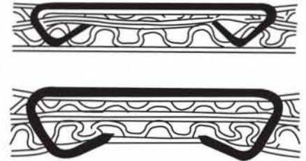
SACA HDCS 19/35 Standart mechanical carton closing stapler
